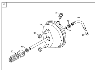
ETB-0000009616, Cylindry membranowe
